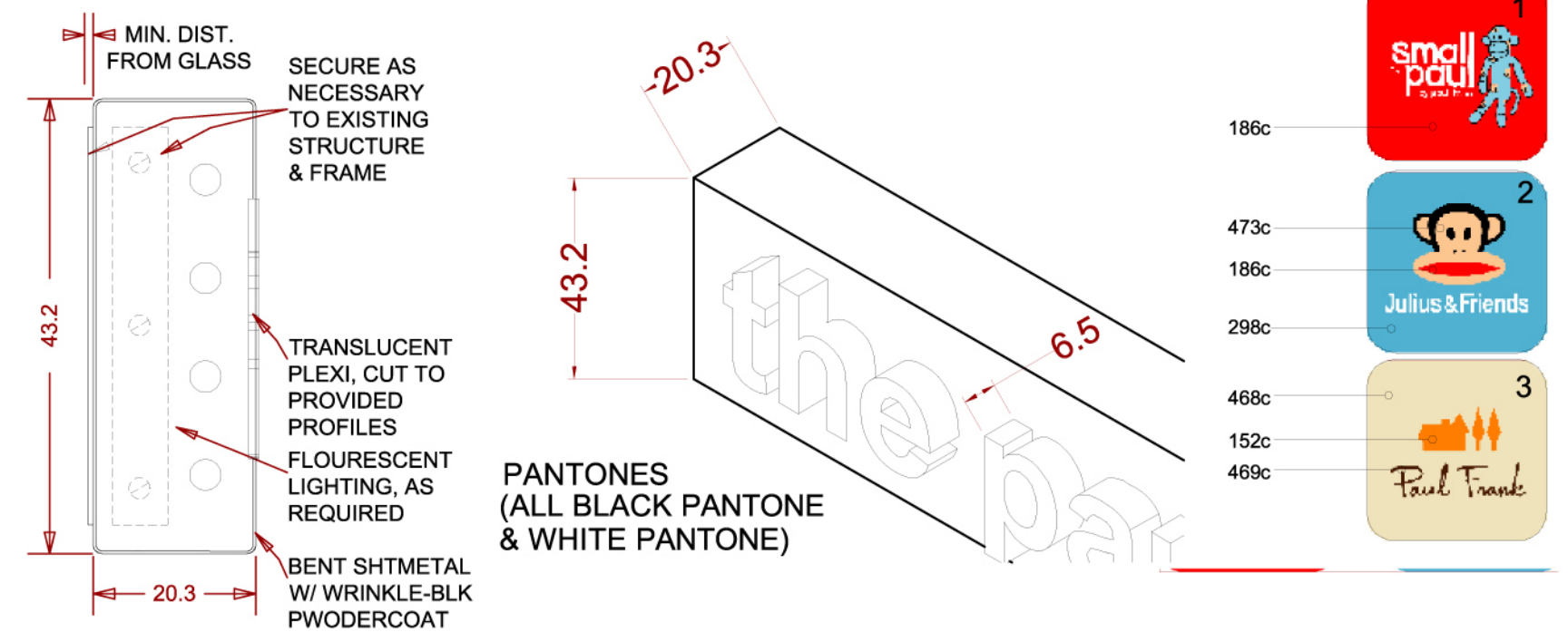
FRONT FACADE SCALE: 1/4"
